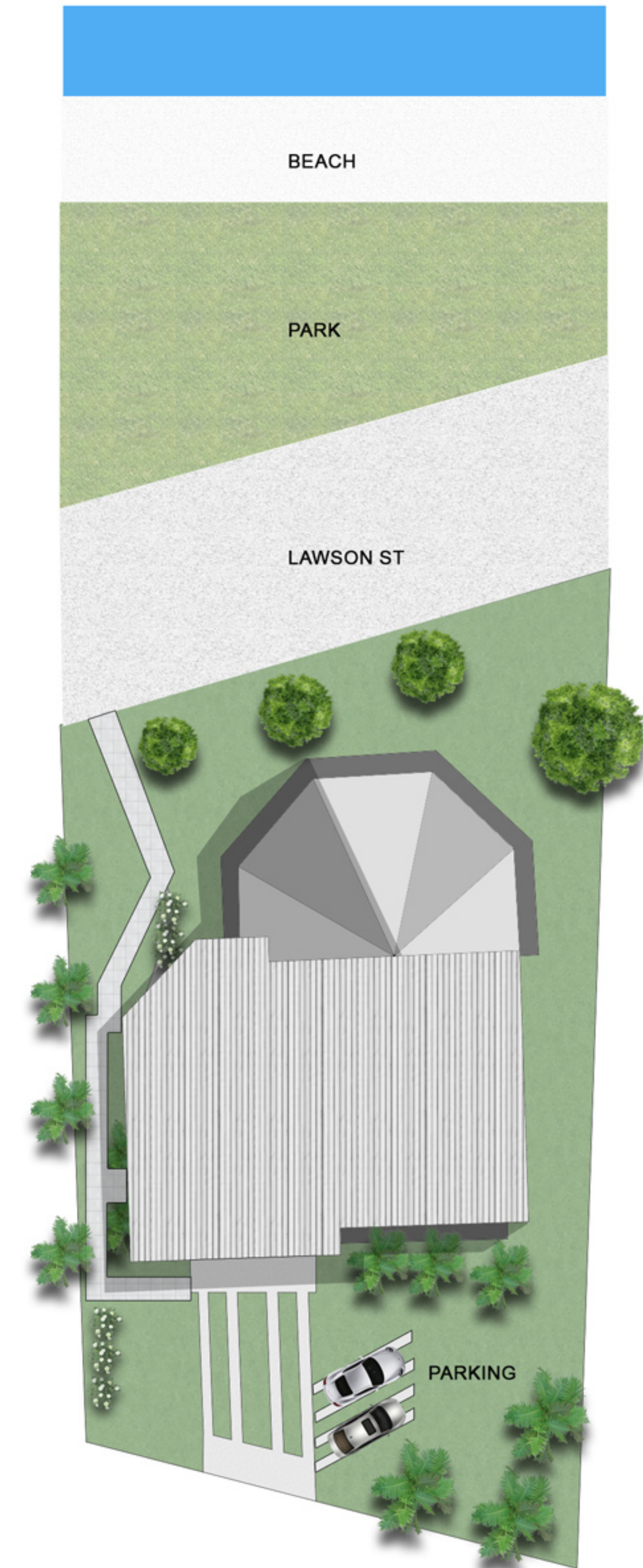
SITE PLAN FIRST FLOOR
